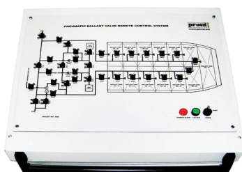
Ballast System Control Panel
